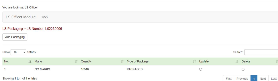
Gambar 12. Interface Packaging
