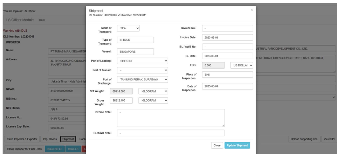
Gambar 11. Interface Shipment
