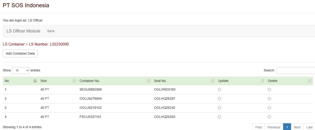
Gambar 16. Interface Container
